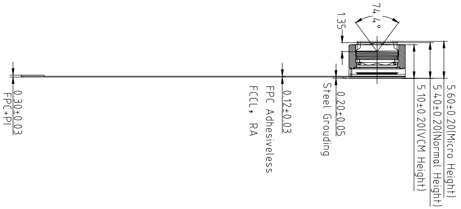
SIDE VIEW
